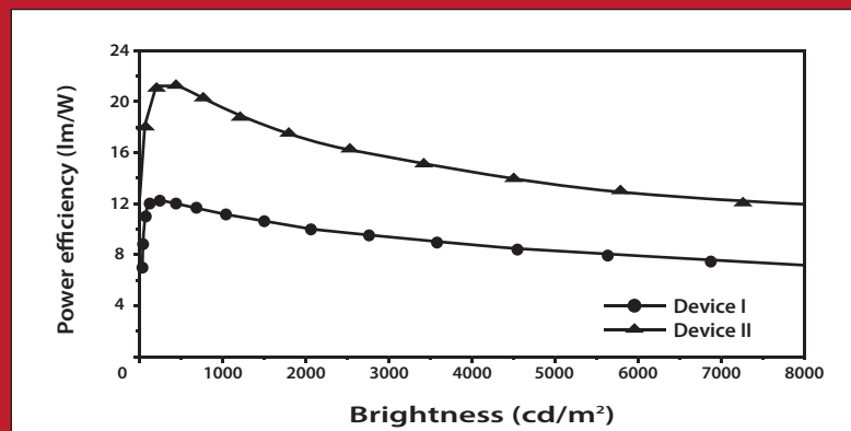
Figure 1 : A comparison of brightness and power efficiency between the OLED and the common LED
