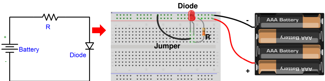
Figure 3. Example of how to place components on a protoboard / breadboard
